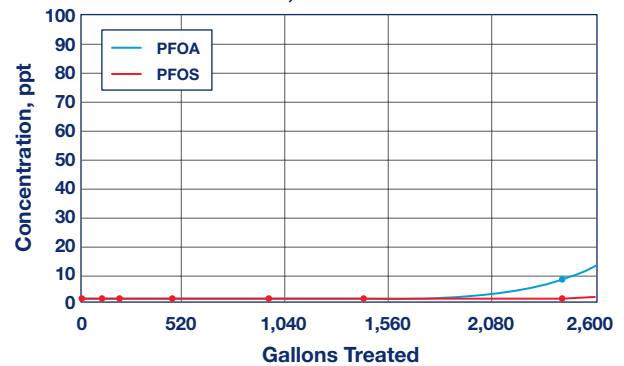
Filter Performance, AF-10-3612-BB for PFOS, PFOA Removal
