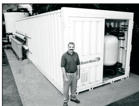
California Water Service Company 1100 GPM Nitrate Removal Unit Jim Luongo – Superintendent of Production
